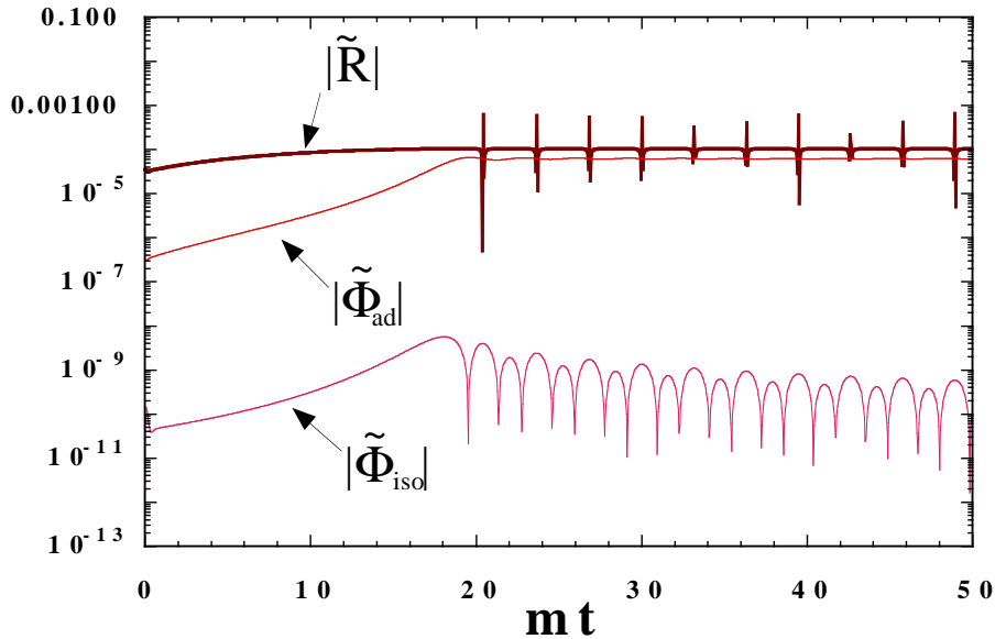
FIG. 1: The evolution of the adiabatic metric perturbation \tilde{\Phi}_{\text{ad}} \equiv k^{3/2}\Phi_{\text{ad}} , the isocurvature metric perturbation \tilde{\Phi}_{\text{iso}} \equiv k^{3/2}\Phi_{\text{iso}} , and the curvature perturbation \tilde{\mathcal{R}} \equiv k^{3/2}\mathcal{R} for the case of \beta = 0.09 in the JBD theory with quadratic inflaton potential, V(\phi) = m^2\phi^2/2 . We choose the initial values of scalar fields as \phi = 3m_{\text{pl}} and \chi = -1.2m_{\text{pl}} , in which case \chi is nearly zero at the end of inflation.
